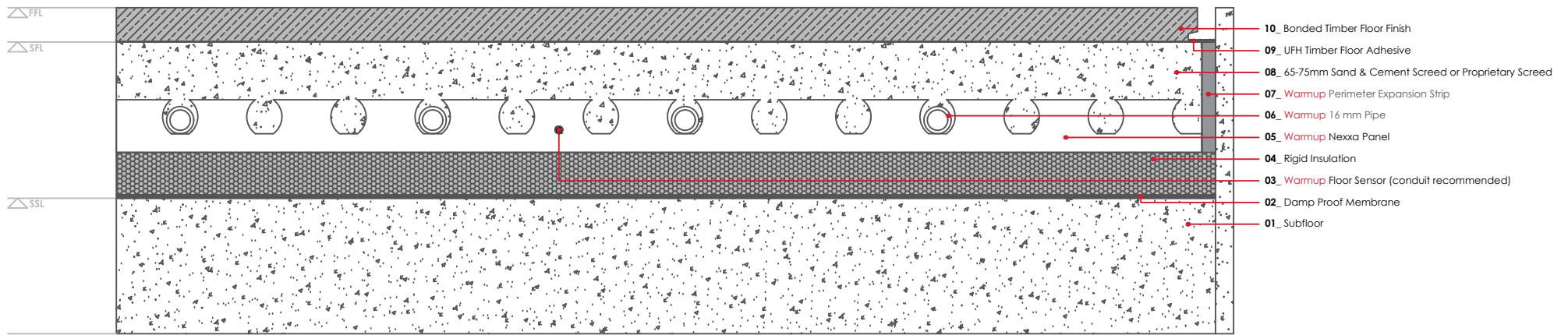
WARMUP Nexxa Bonded timber floor finish
