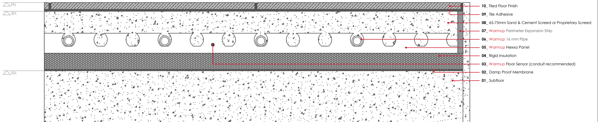
WARMUP NEXXA SYSTEM. Tiled floor finish
