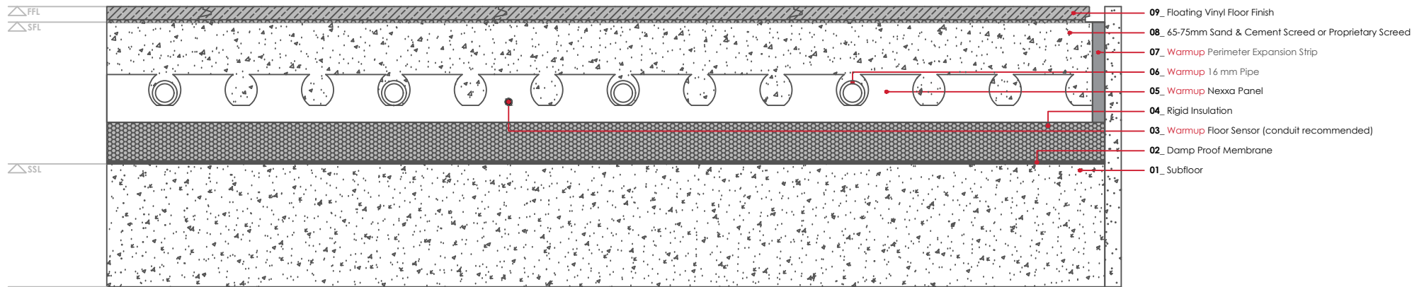
WARMUP Nexxa SYSTEM. Vinyl floor finish - floating
