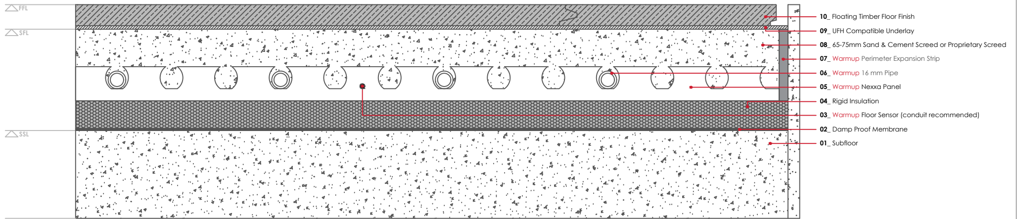
WARMUP Nexxa Floating timber floor finish
