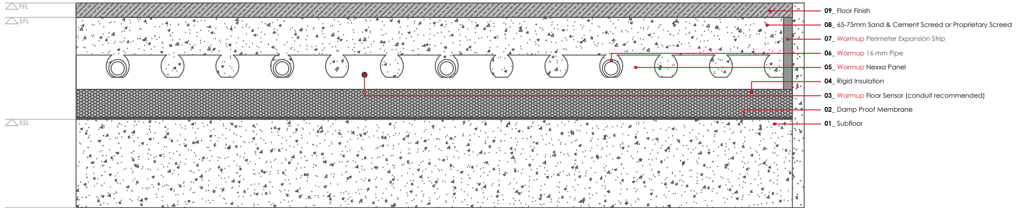
WARMUP NEXXA SYSTEM. Standard Detail
