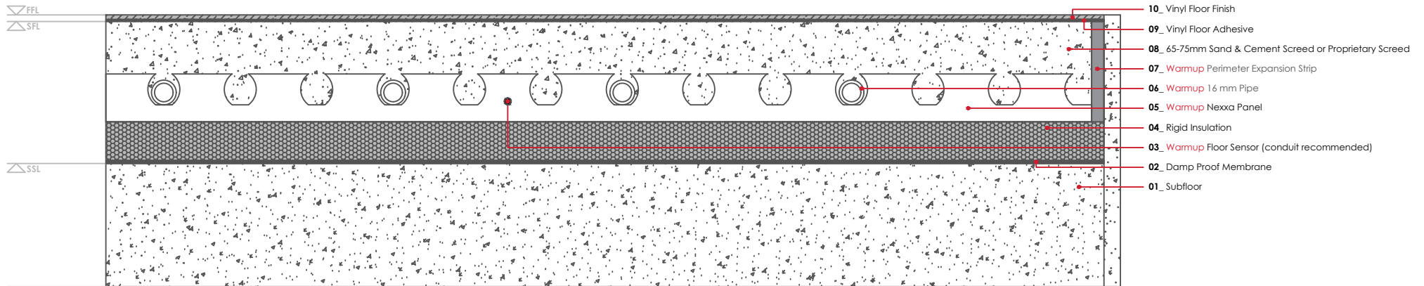
WARMUP Nexxa SYSTEM. Vinyl floor finish - glued
