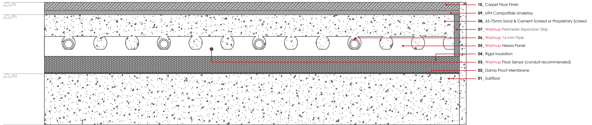
WARMUP Nexxa SYSTEM. Carpet floor finish
